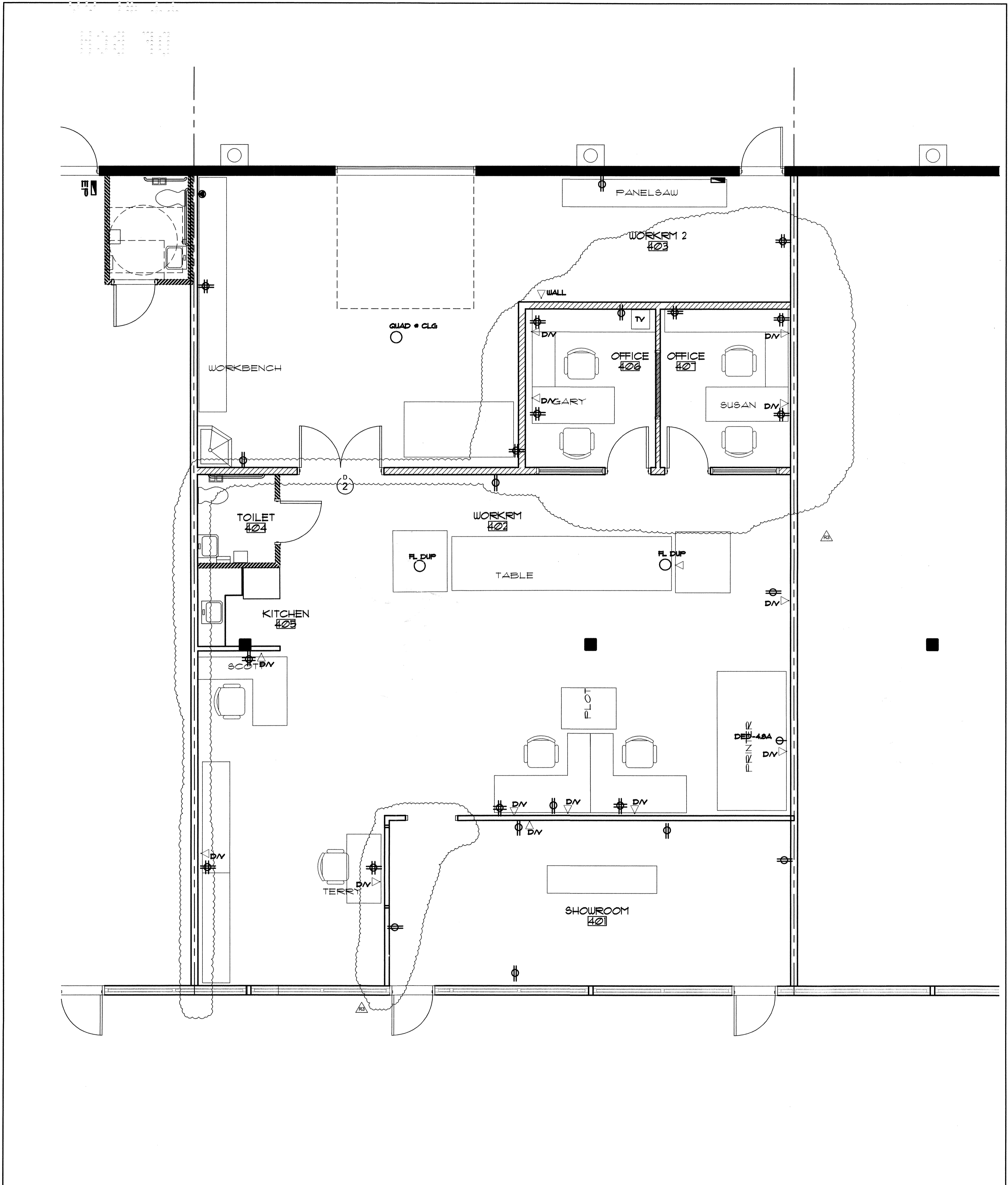
1 FURNITURE & ELECTRIC PLAN SCALE: 3/32" = 1'-0"
